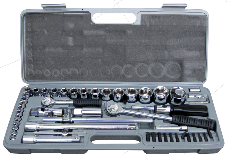
Special tool box (No. 200 200) for closing of CO 2 -cartridges
